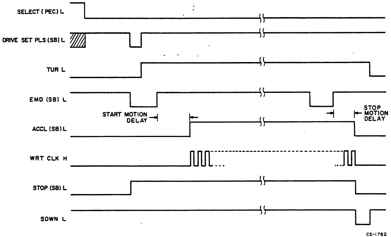
Figure 4-3 Starting and Stopping Interrelationships
